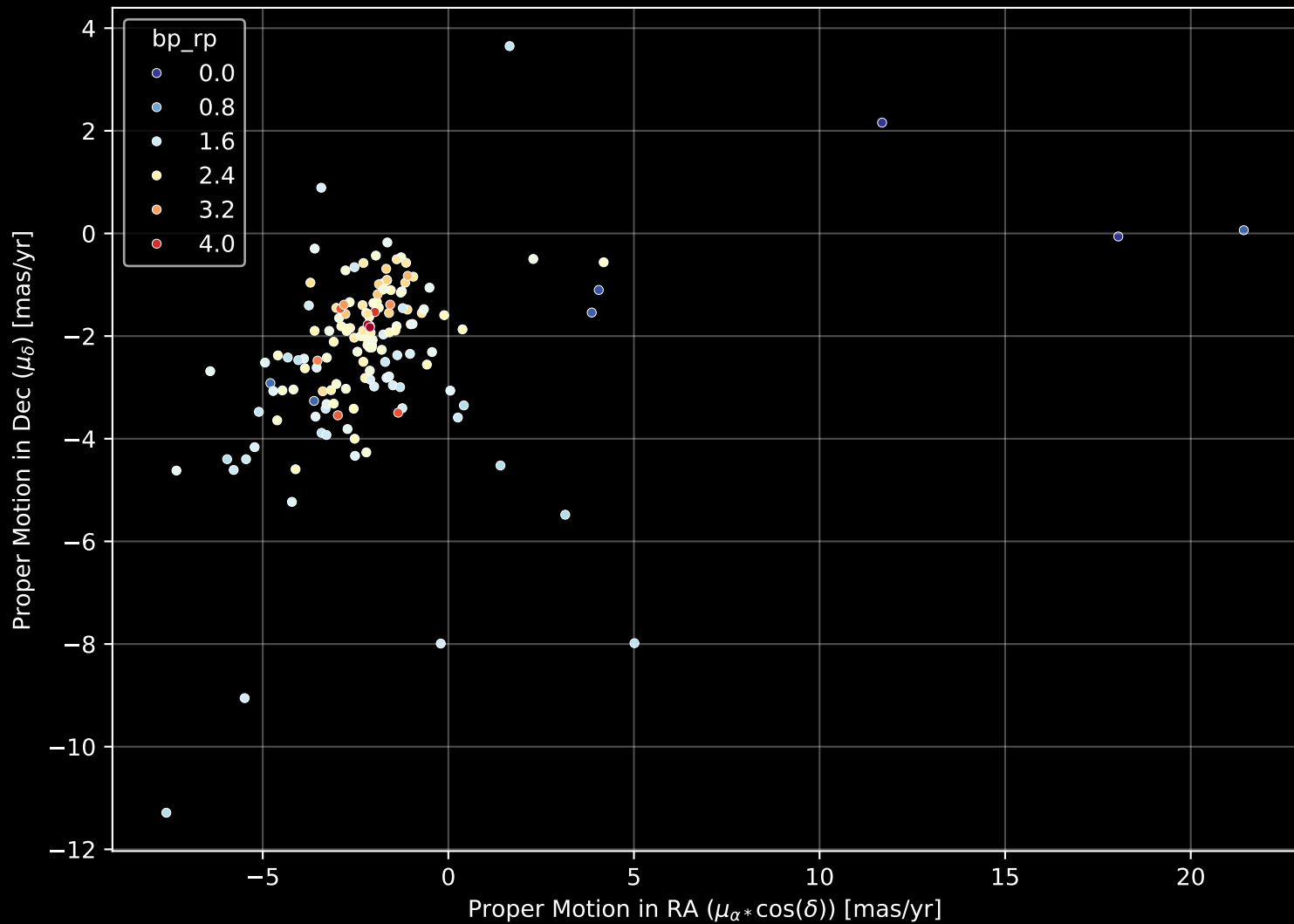
APOGEE DR17 Field: [Lac_2] Proper Motion Diagram (n= 151)
