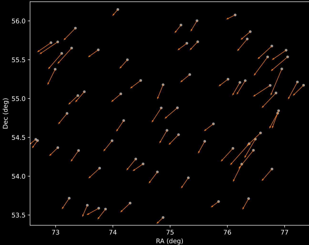
APOGEE DR17 Cluster 2 Proper Motion Vectors (n=69)
