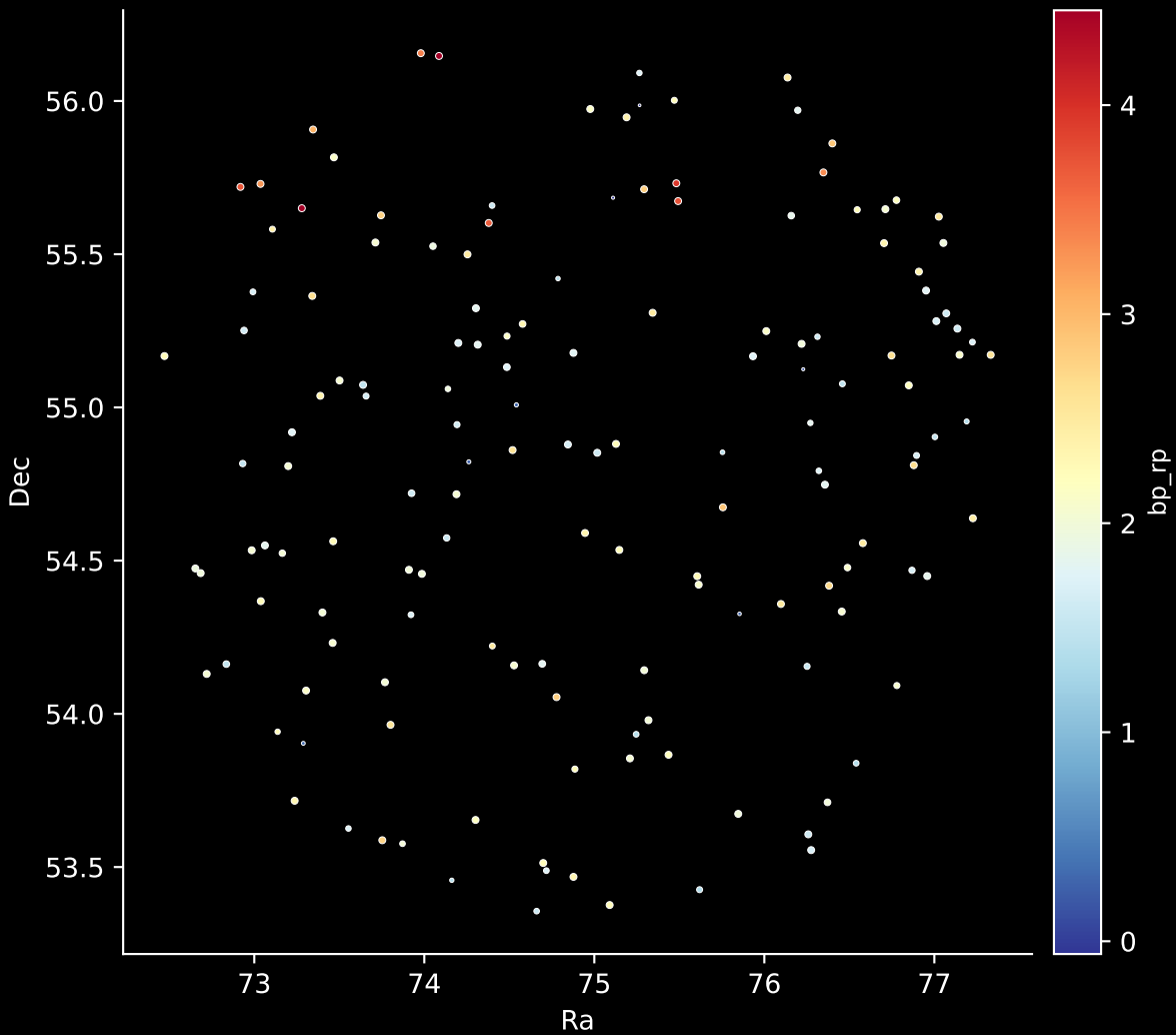
APOGEE DR17 Field: [Lac_2] Stars: 151
