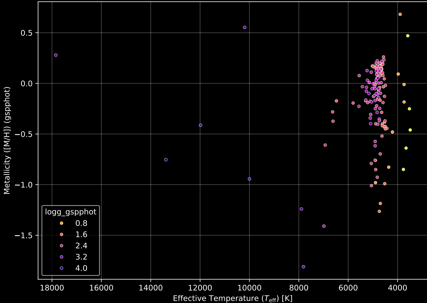
APOGEE DR17 Field: [Lac_2] Stellar Population Parameters (n= 151)
