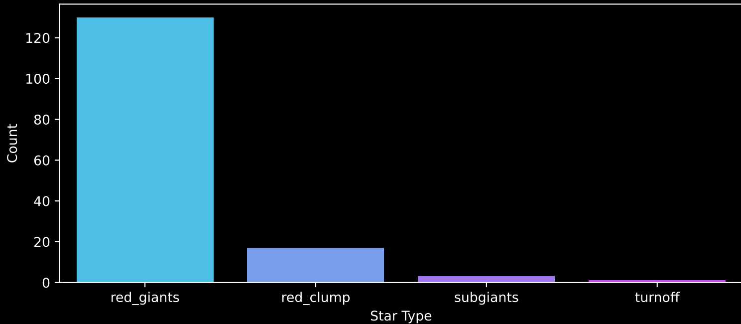
APOGEE DR17 Field: [Lac_2] Count plot of Star Type
