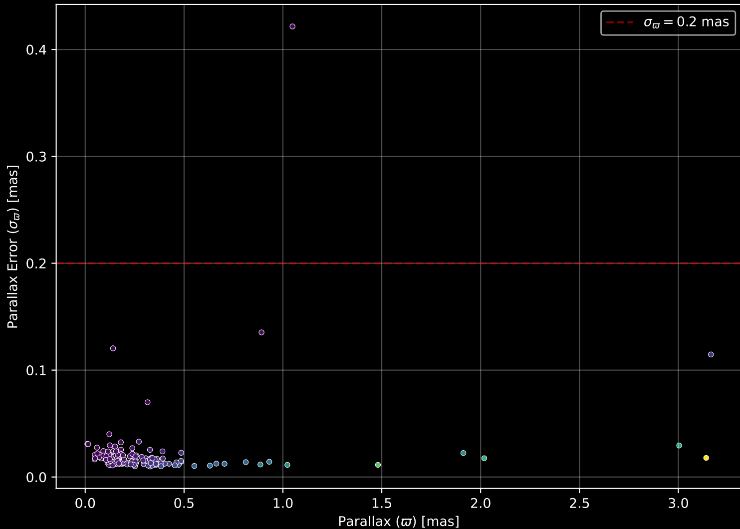
APOGEE DR17 Field: [Lac_2] Parallax Quality (n= 151)
