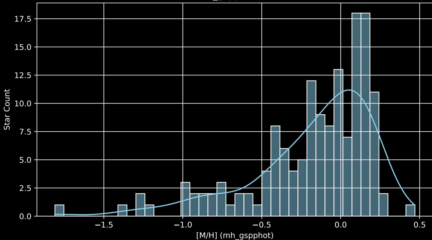
APOGEE DR17 Field: [Lac_2 [M/H] (mh_gspphot) (n= 149)
