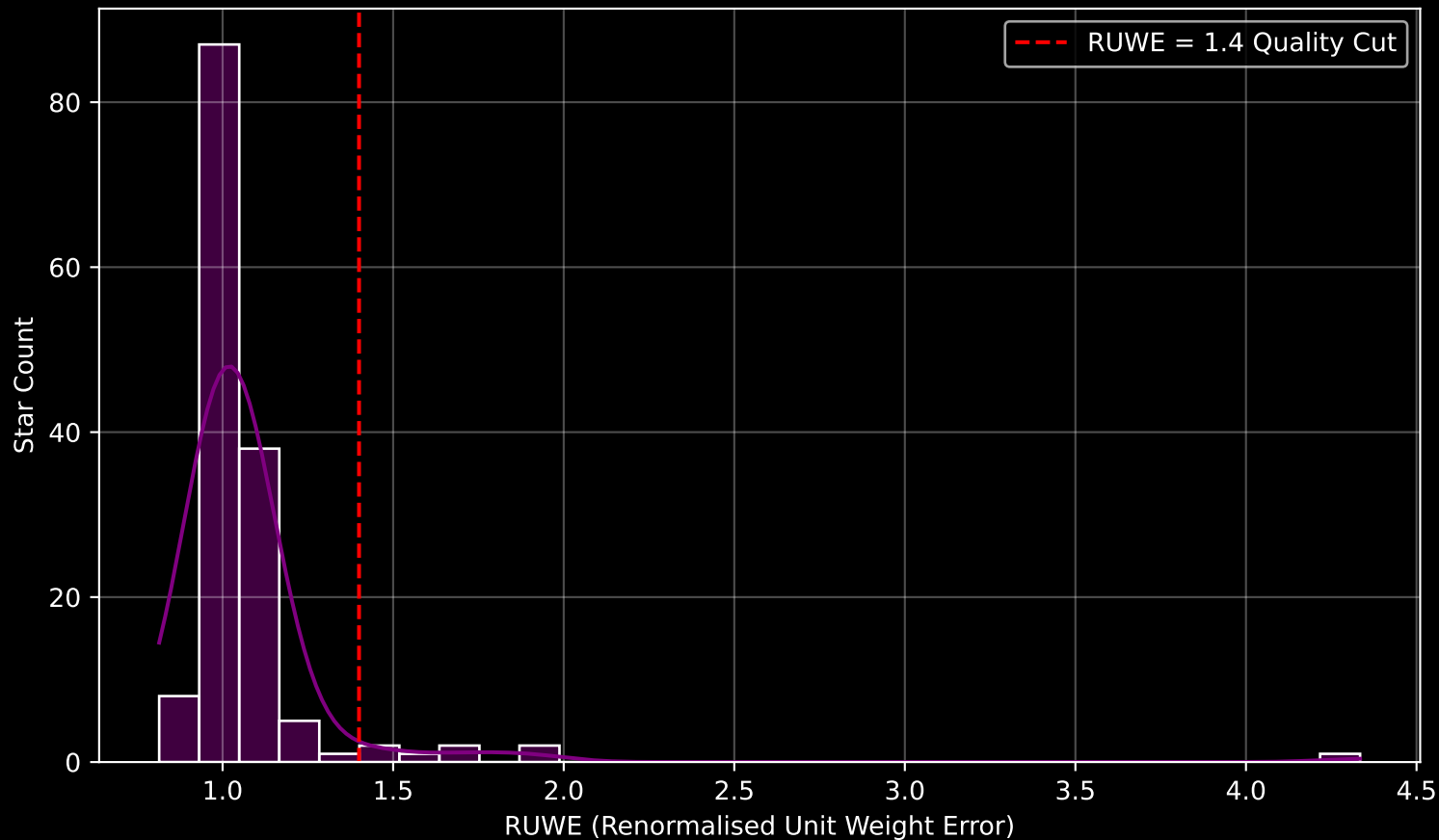
GAPOGEE DR17 Field [Lac_2] RUWE Distribution (n= 147)
